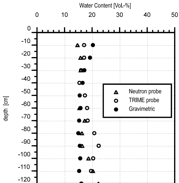
Figure 3: Comparison of neutron probe, TRIME-T3 and gravimetric method for water content determinations in a loess soil.
