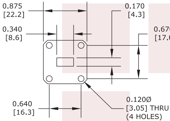
UG 1530/U WR 34 COVER FLANGE
