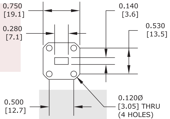
UG 599/U WR 28 COVER FLANGE
