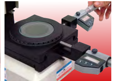
X-Y measuring table and micrometer head.
