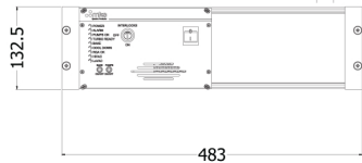
FRONT VIEW ON RVC/DSU/SUBRACK
