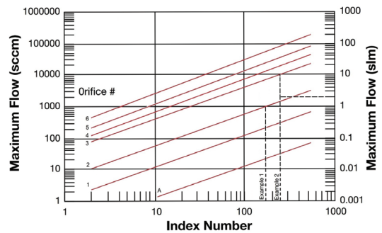
Figure 2 — Orifice Selection Graph (See Note)
