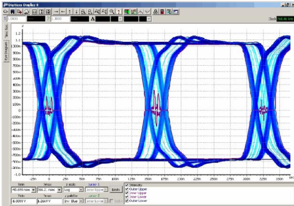
Eye diagram
