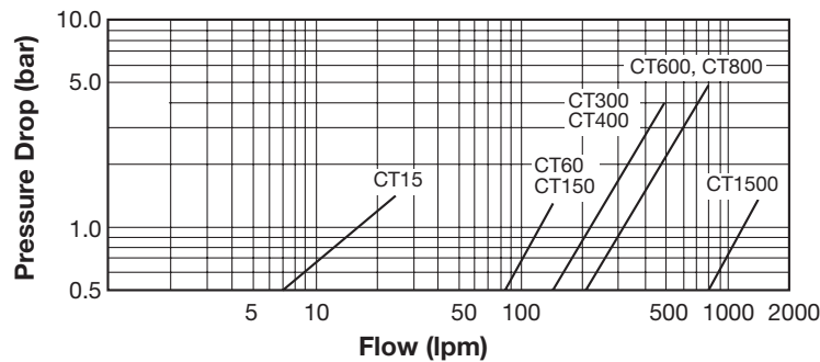
Pressure Drop Chart Hydraulic Oil Viscosity 21 Centistokes
