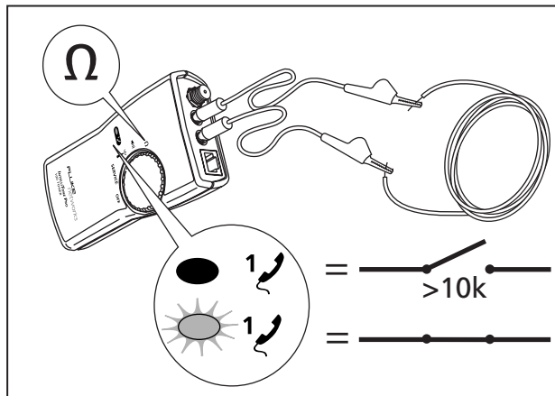
Figure 3. Continuity Test
