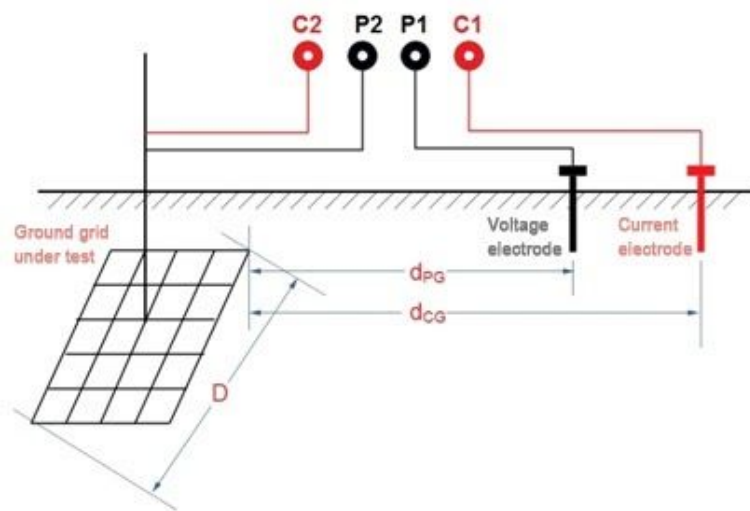
Wiring method 1
