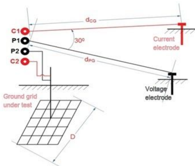
Wiring method 2
