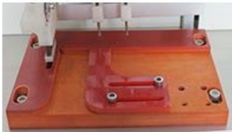
Test Fixture Can adjust position for battery
