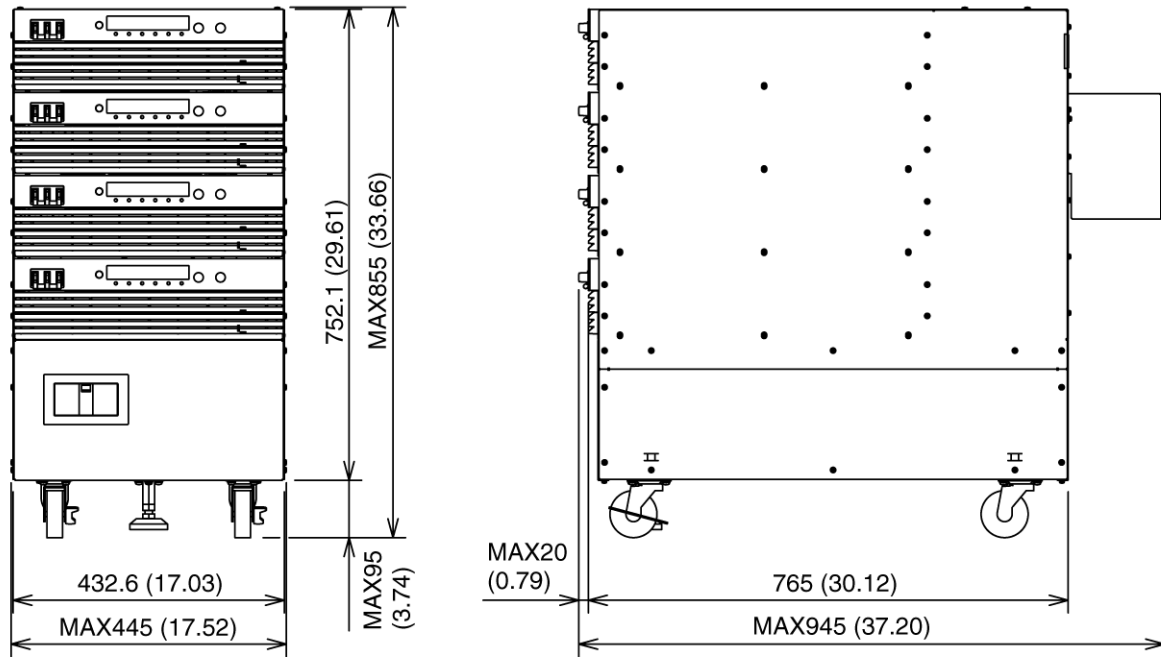
PAT-TMX Series 32 kW System Outline Drawing
