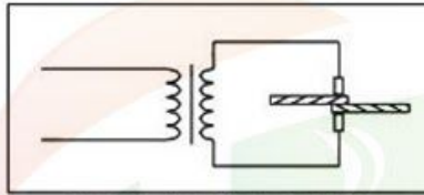
Touch-welding profile
