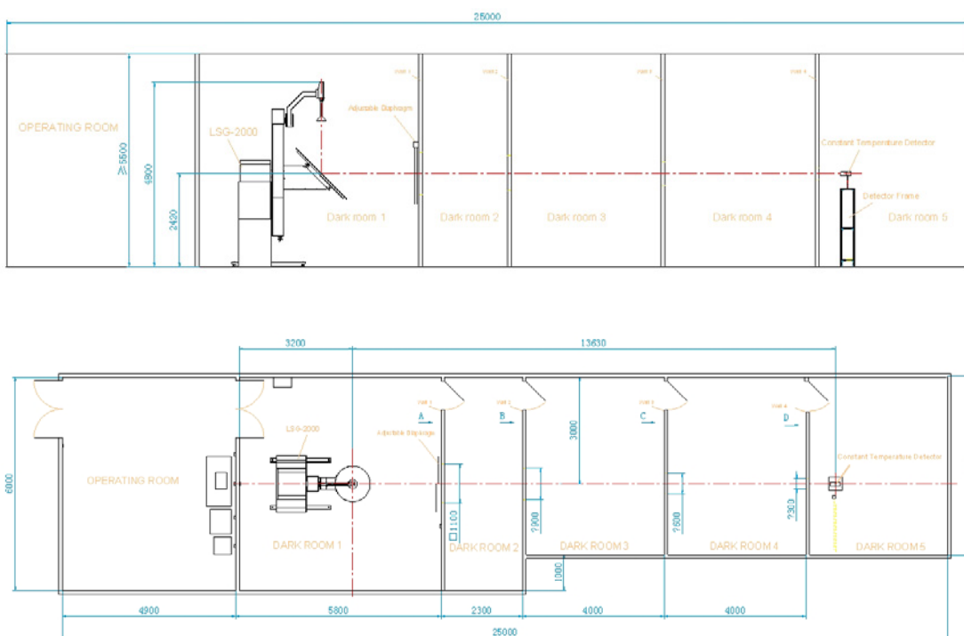
Fig: LSG-2000CCD lab dark room view
