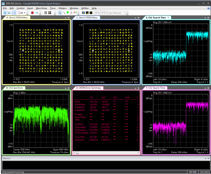
Figure 4. Example of a 2-channel, 400 MHz analysis.
