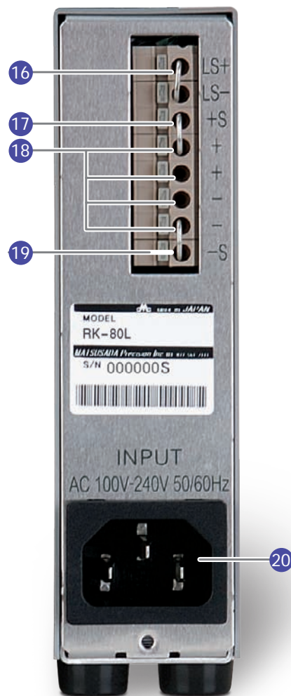
Rear panel
