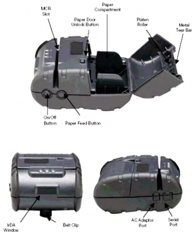
FIGURE 1: PRINTER OVERVIEW
